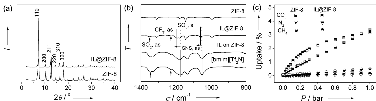
Figure 1. PXRD patterns (a) and ATR-FTIR spectra (b) of ZIF-8 and IL@ZIF-8. c) Adsorption isotherms of CO 2 , N 2 and CH 4 on ZIF-8 and IL@ZIF-8 at 298 K.
